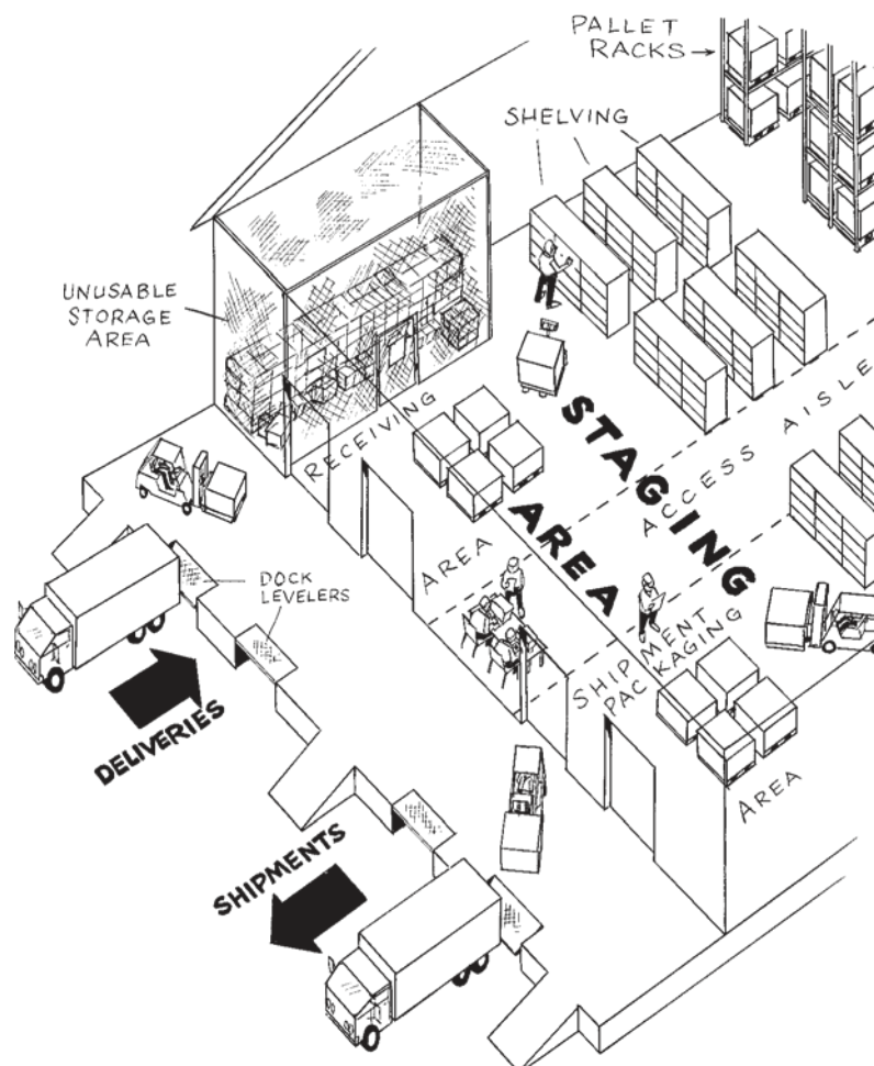
Figure 1. Typical Layout for Receiving/Shipping Activities
